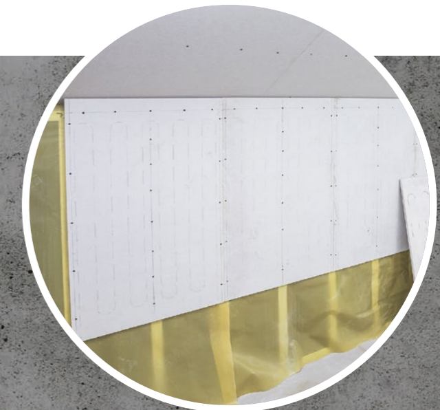
Fastening with clamps to a load-bearing wooden structure
