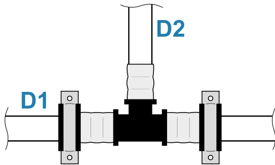
Example of execution of a fixed point next to a branch-off of a KAN-therm ultraLINE, ultraPRESS and Push system pipeline
