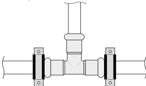
Example of execution of a fixed point next to a branch-off of a KAN-therm Steel/Inox/Copper.
