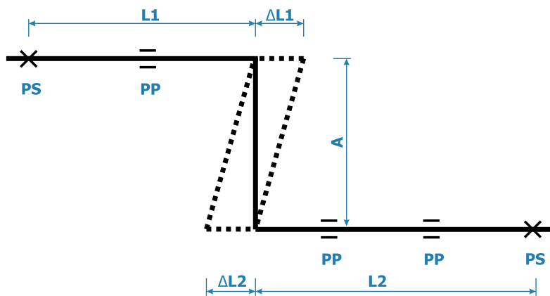
Type Z compensator
