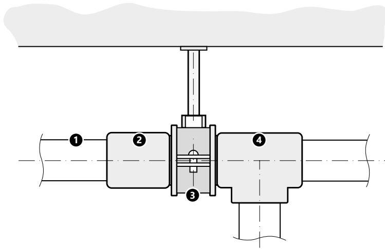
Example of execution of a fixed point next to a branch-off of a KAN-therm PP system pipeline
