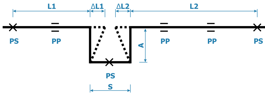
U-type compensator
