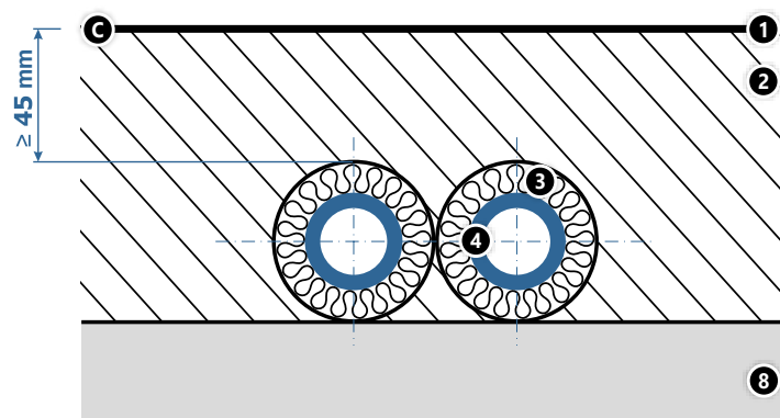
C. Directly on concrete mortar
